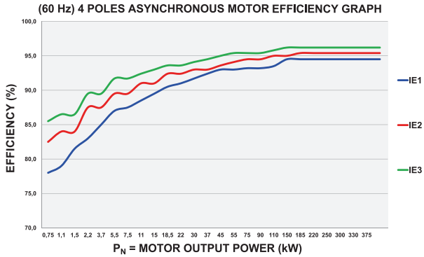
FIGURE 7: 4 poles Asynchronous motor efficiency power chart (60Hz)
