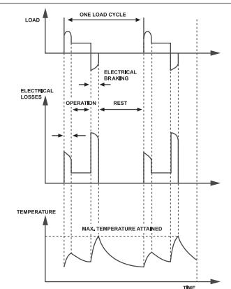
FIGURE 14: S-5 DUTY TYPE - Intermittent periodic duty with electric braking
