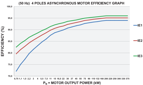
FIGURE 4: 4 poles Asynchronous motor efficiency power chart (50 Hz)
