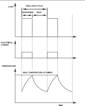
FIGURE 12: S-3 DUTY TYPE - Intermittent periodic duty
