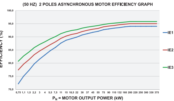
FIGURE 3: 2 poles Asynchronous motor efficiency power chart (50 Hz)
