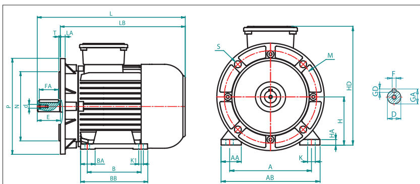
FIGURE 50: Asynchronous three-phase motors, aluminum housing, foot mounted, B35
