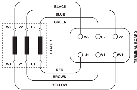
FIGURE 28: Connection of stator winding ends to the terminal table
