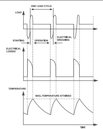
FIGURE 16: S-7 DUTY TYPE - Continuous operation periodic duty with electric braking
