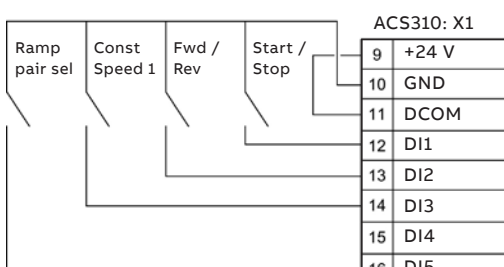
DI configuration NPN connected (sink)
