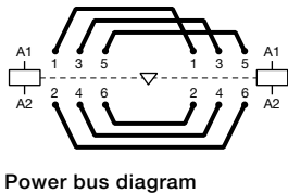
Power bus diagram
