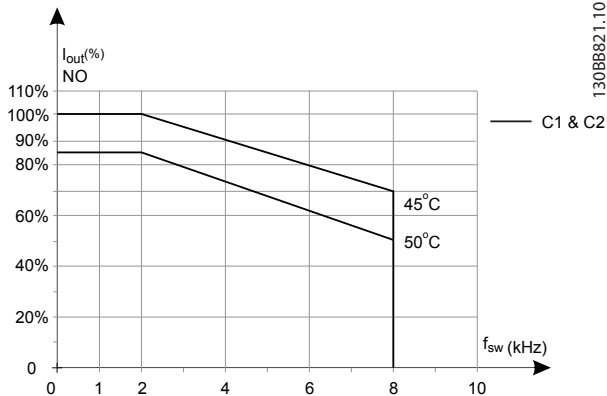
Illustration 5.19 Output Current Derating with Switching Frequency and Ambient Temperature for 600 V Frequency Converters, Enclosure Sizes C, 60 AVM, NO
