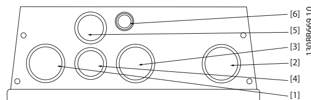
Illustration 8.28 Enclosure Size B1, IP55
