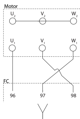
Illustration 3.10 Terminal Connection for Clockwise and Counter-clockwise Rotation
