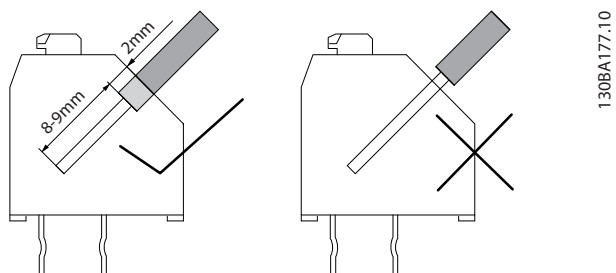
Illustration 7.15 Mounting of Cables
