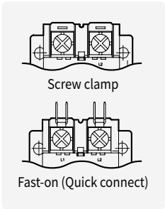
Main terminal
