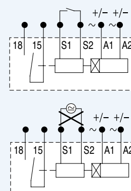
Circuit diagram
