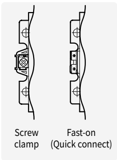
Coil terminal
