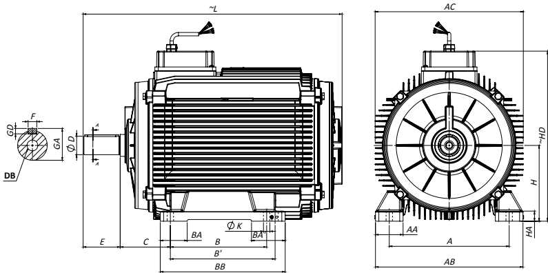
FOOT MOUNTED MOTOR (IEC 60072-1) - B3
