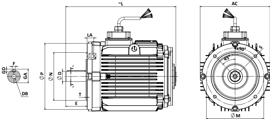
FLANGED MOTOR (FORM “C” - IEC 60072-1) - B14-2, V18, V19
