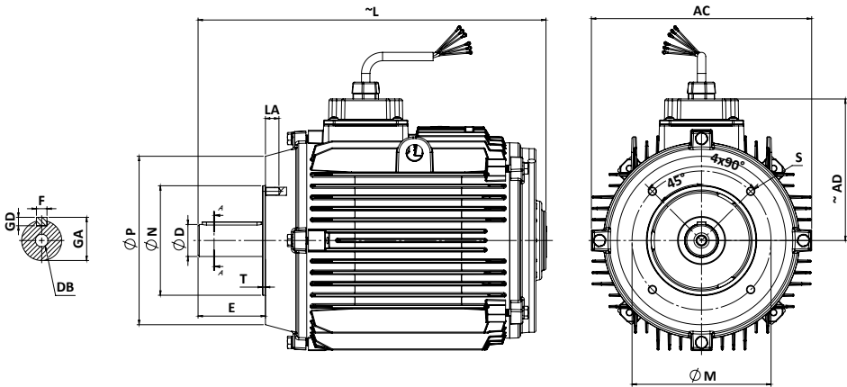
FLANGED MOTOR (FORM “C” - IEC 60072-1) - B14, V18, V19
