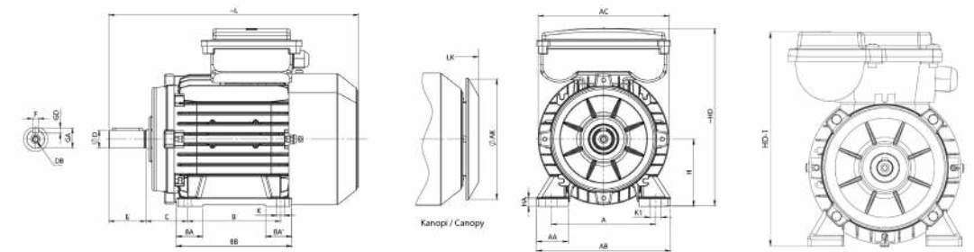
FOOT MOUNTED MOTOR (IEC 60072-1) - B3, B6, B7, B8, V5, V6
