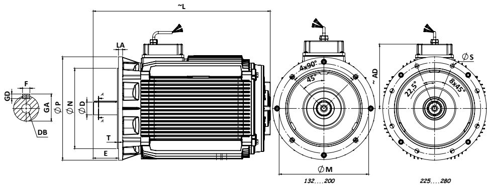
FLANGED MOTOR (FORM “A” - IEC 60072-1) - B5, V1, V3
