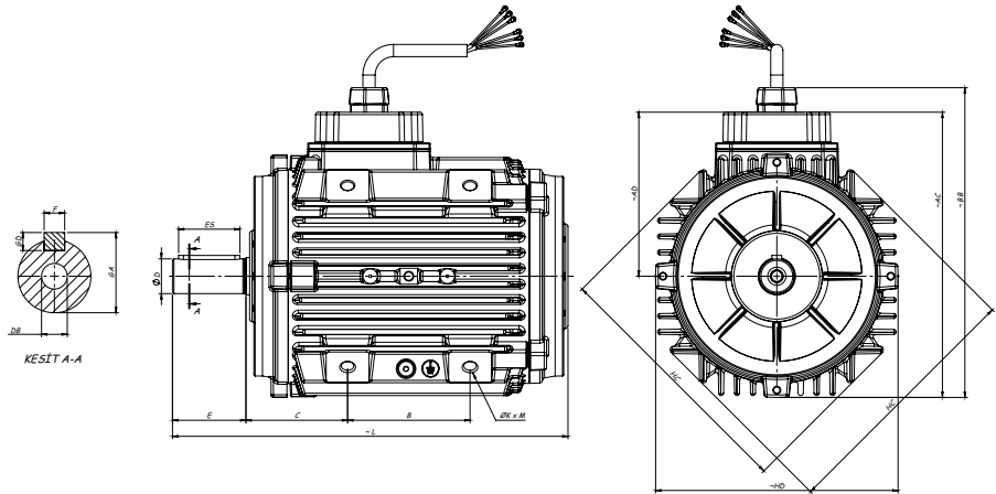
PAD MOUNTED SMOKE EXTRACTION MOTORS (FORM “C” - DIN EN 60072-1) - B30
