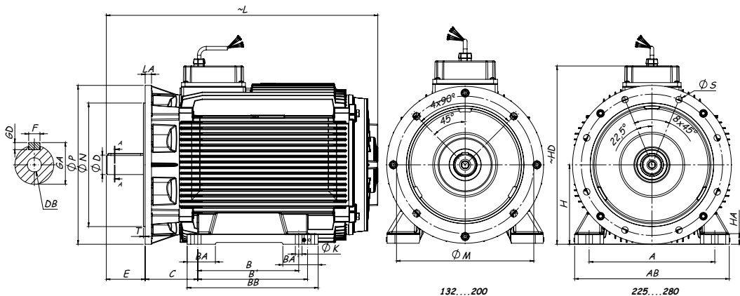
FOOT MOUNTED AND FLANGED MOTOR (FORM “A” - IEC 60072-1) - B35
