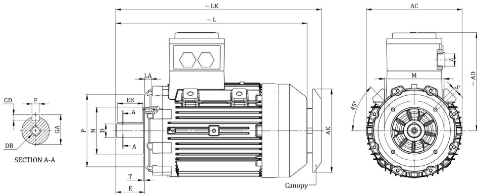
FLANGED MOTOR (FORM C) - B14, V18, V19
