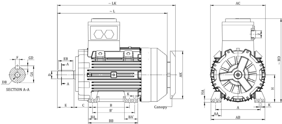
FOOT MOUNTED MOTOR - B3, B6,B7, B8, B15, V5, V6
