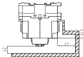
Insulation Distance
