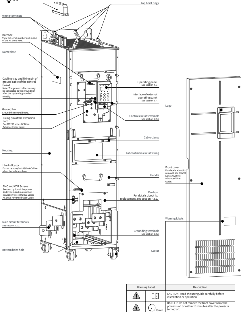
Figure 1-3 Components (Three-phase 380–480 V, MD290T200G to MD290T450G, MD290T220P to MD290T500P)
