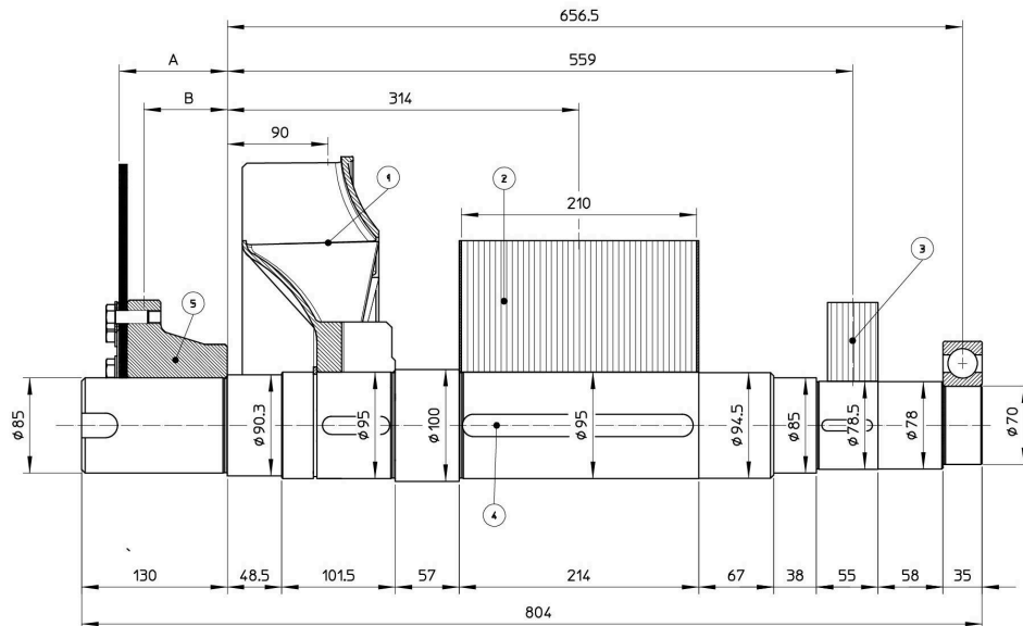
5 SHAFTS COUPLING FLEX PLATE
