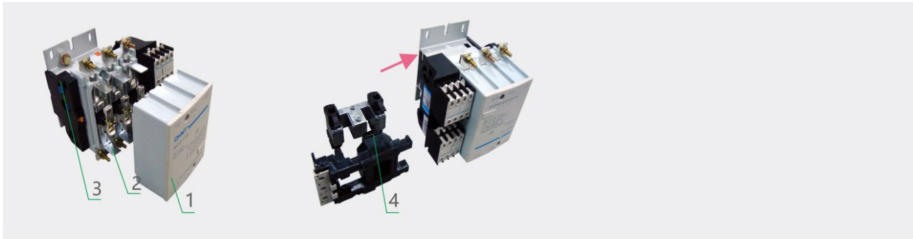
1:arc-extinguishing system 2:contact system 3:base frame 4:magnetic system
