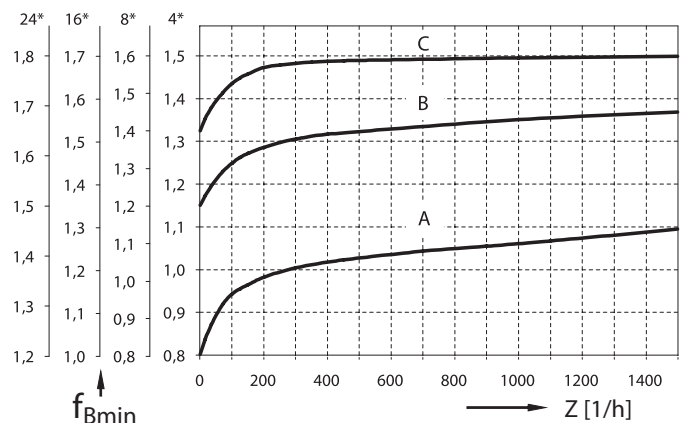
Diagram 1: Minimum service factor f_{Bmin}
