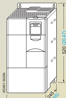
Inverter frame size D
