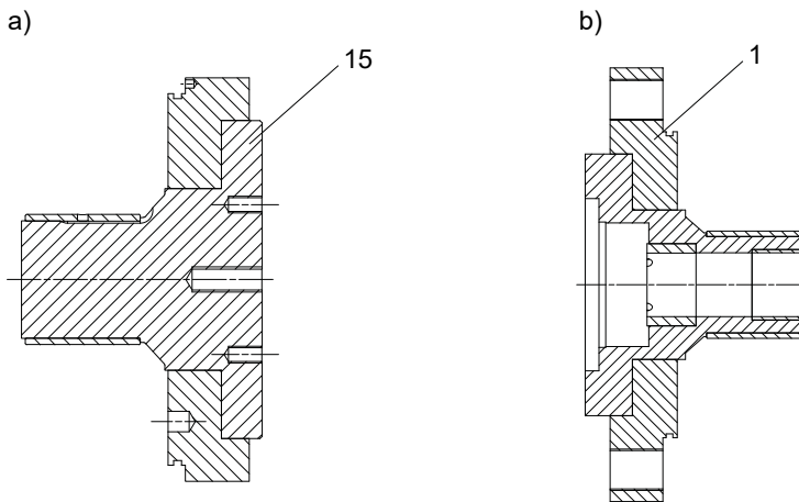
Detailed view: a) end cover b) Pump flange
