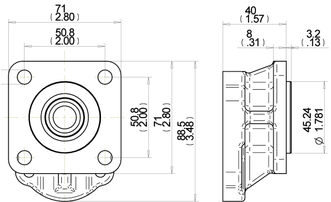
S1 SAE AA 4 bolts
