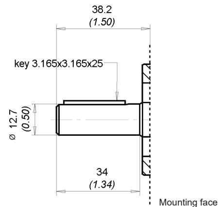
code 83 Max torque 40 Nm (354 lbf in) SAE Parallel
