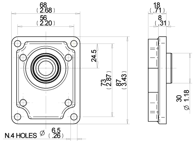
P01 European standard
