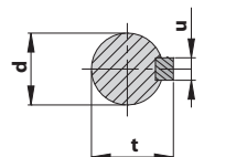
SHAFT DIMENSIONS
