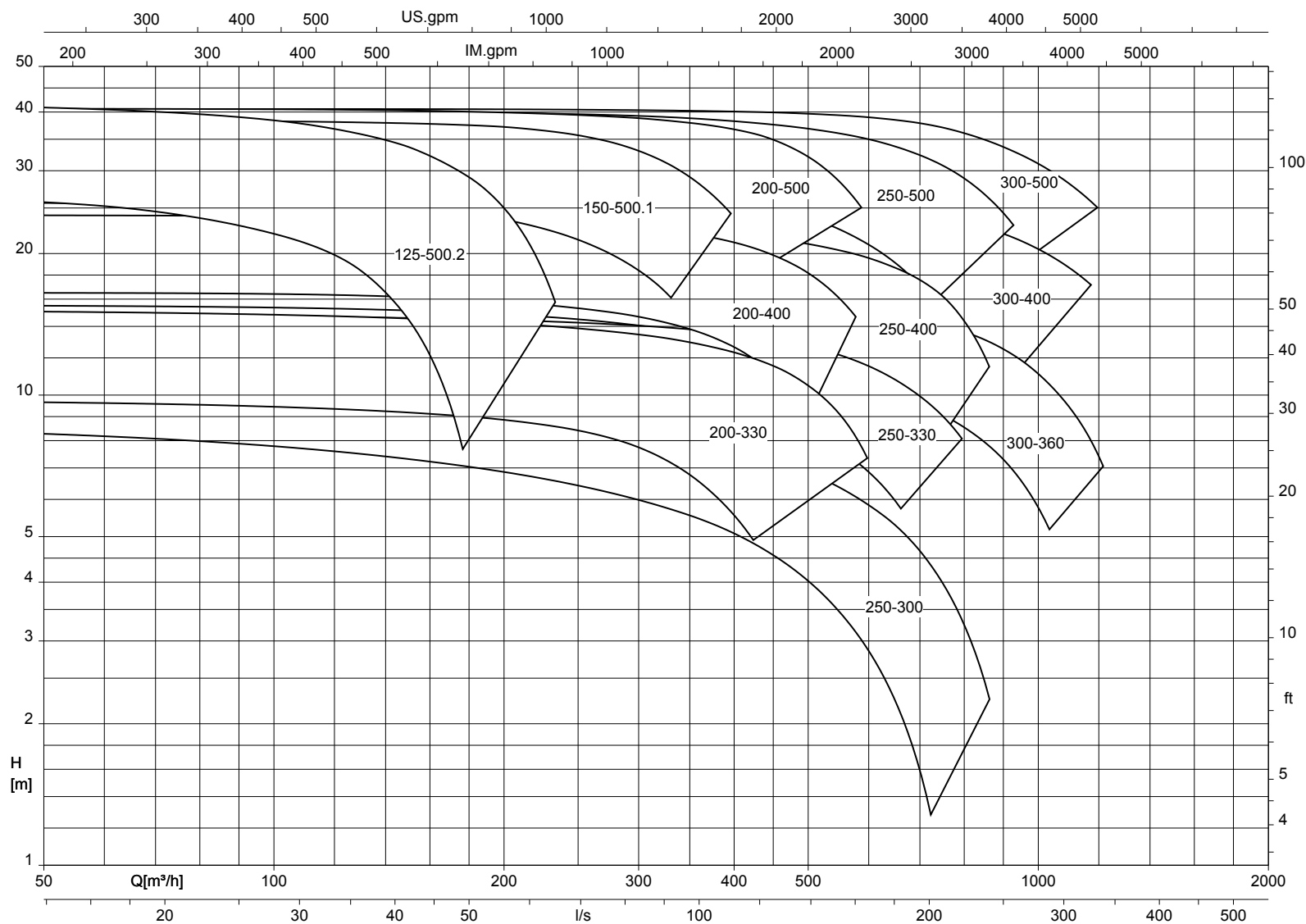
Etanorm-RSY, n = 960 rpm
