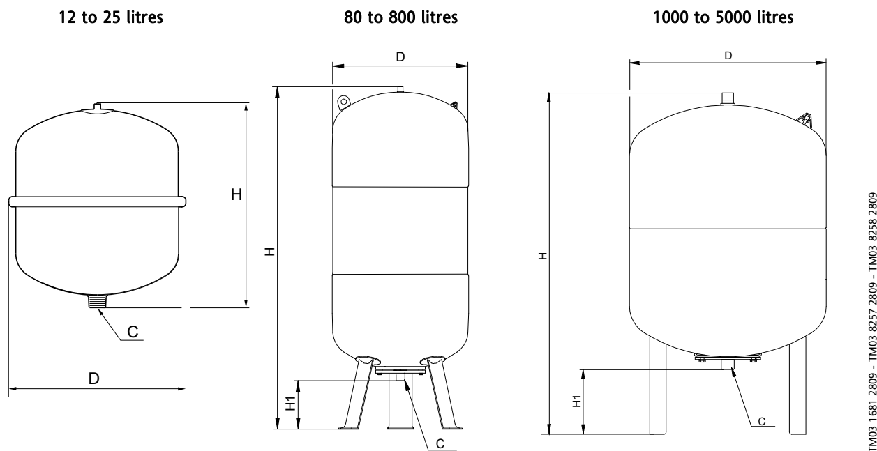
Fig. 7 Dimensional sketches
