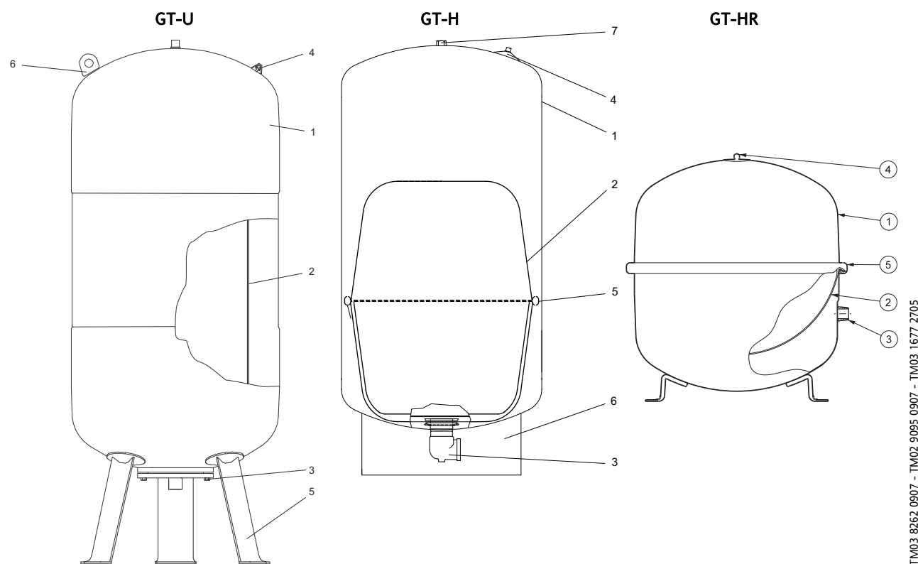
Fig. 1 Sectional drawings, examples of tanks. The actual GT tank may look different from the examples shown.
