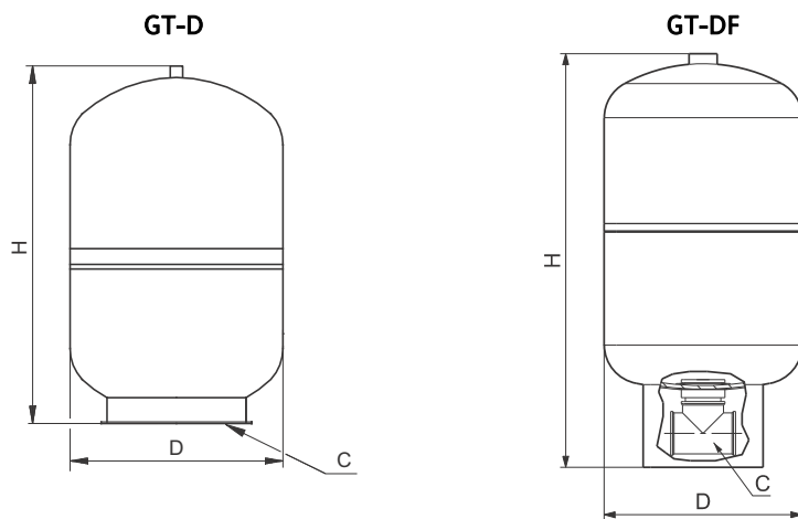
Fig. 12 Dimensional sketches
