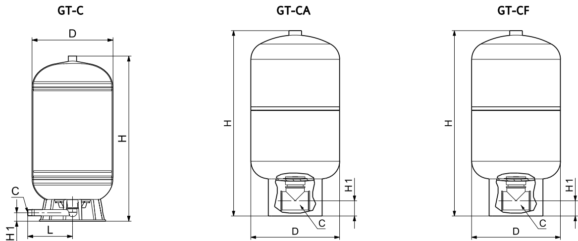
Fig. 13 Dimensional sketches
