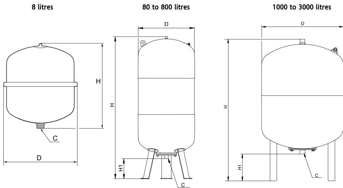
Fig. 8 Dimensional sketches
