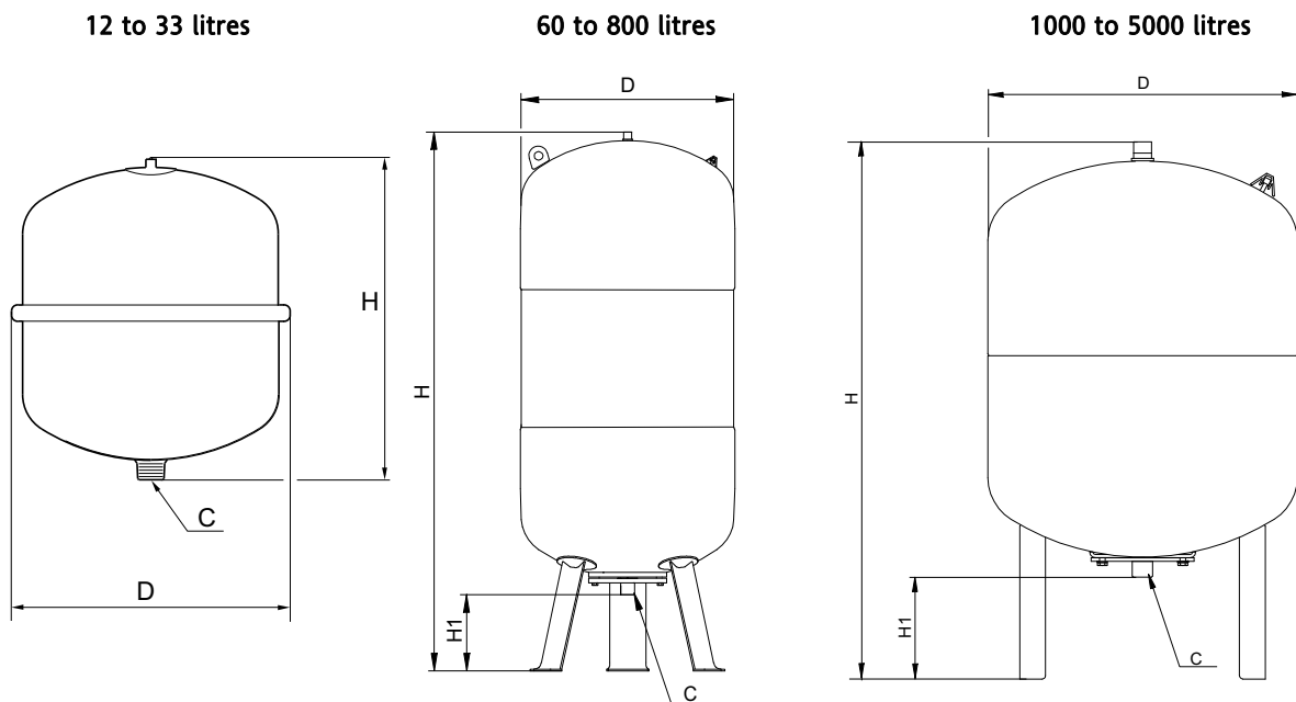
Fig. 6 Dimensional sketches
