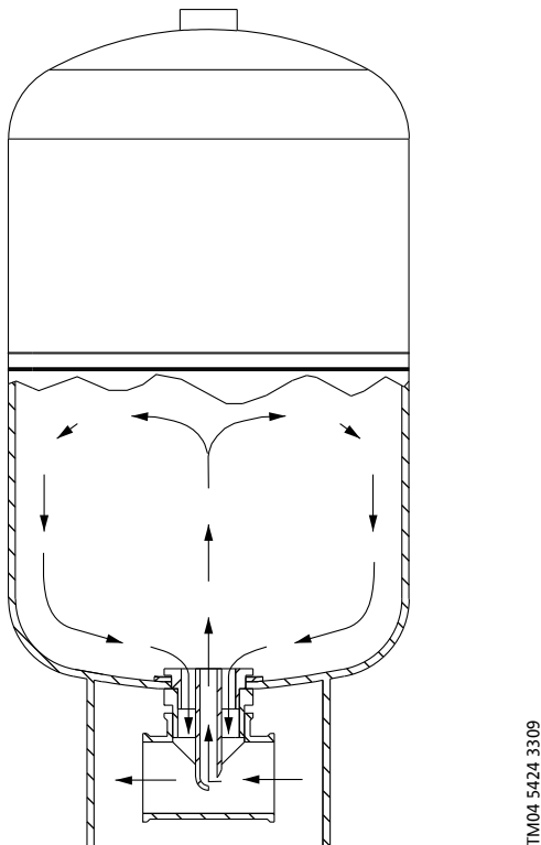
Fig. 3 Illustration of the FlowThru principle
