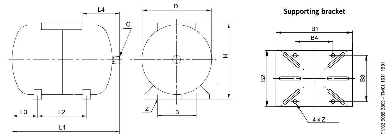
Fig. 11 Dimensional sketches
