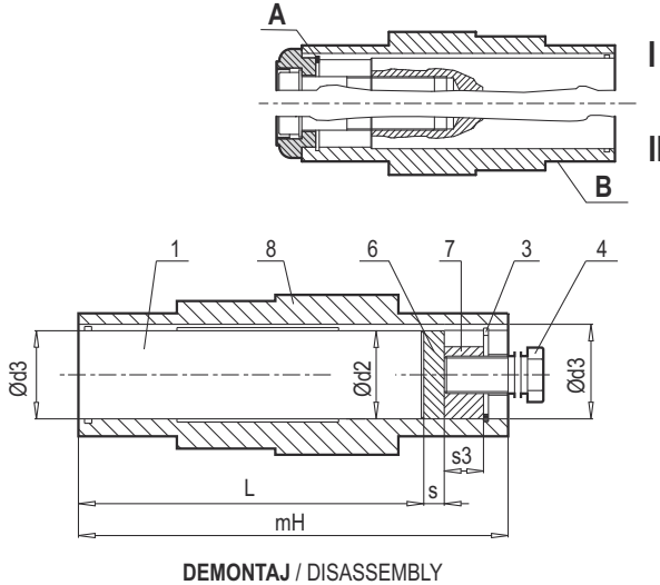
DEMONTAJ / DISASSEMBLY
