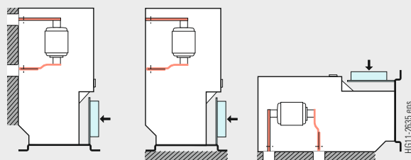
Wall mounting Vertical arrangement
