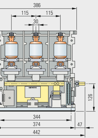
3TL8 dimension drawing
