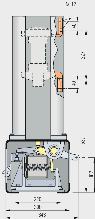
3TL7 dimension drawing
