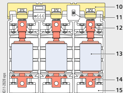
Construction of the 3TL6 vacuum contactor (front view)
