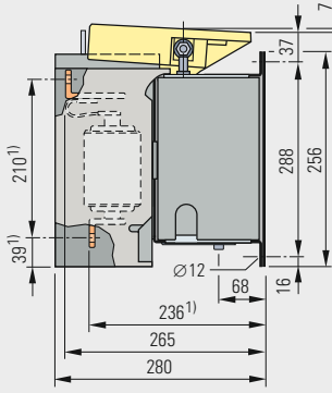
3TL61 dimension drawing
