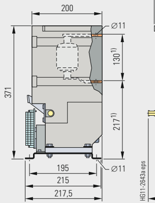
3TL8 dimension drawing
