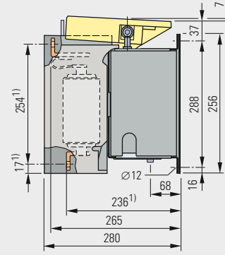
3TL65/68 dimension drawing
