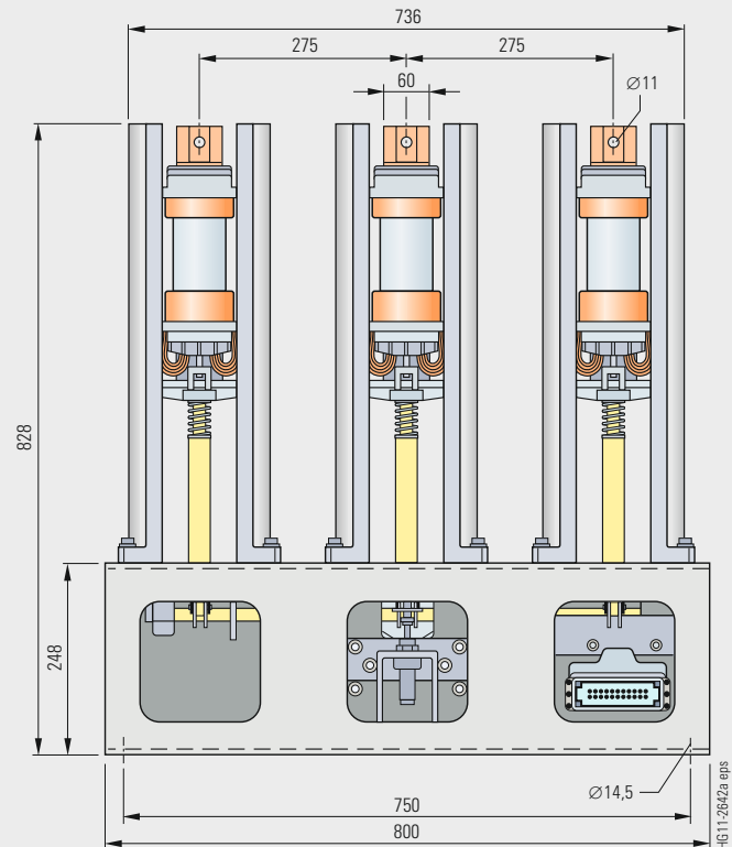
3TL65/68 dimension drawing
