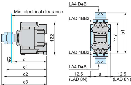
LC1 D40A...D65A (3-pole), LC1 DT60A...DT80A (4-pole)
