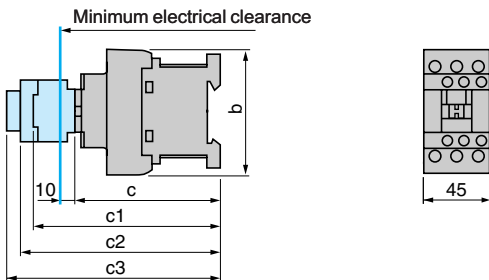
LC1 D25...D38 (3-pole)
