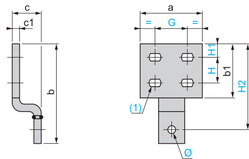
Right-angled connectors LA9 F2100 (set of 6) for rear connection
