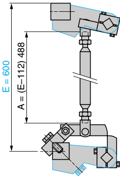
Mechanical interlock for assembling vertically mounted reversing contactors EZ2 LB0601
