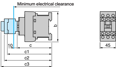
LC1 DT20...DT40 (4-pole)
