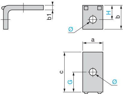
Right-angled connectors LA9 F●979 (set of 3) for side connection
