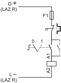
LAZ R9●● + LC1 D
