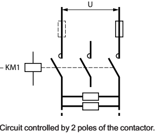
Circuit controlled by 2 poles of the contactor.
