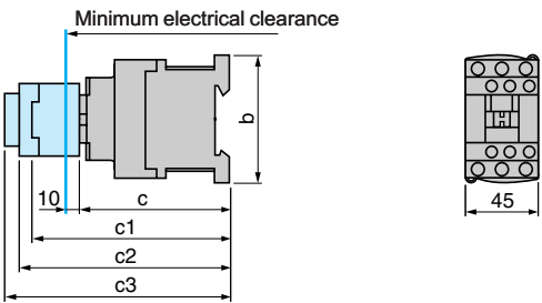
LC1 D09...D18 (3-pole)
