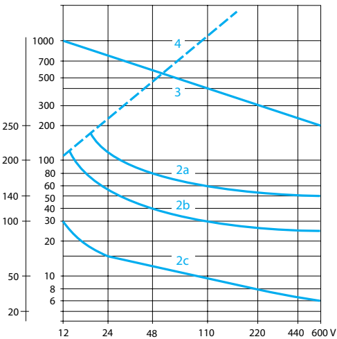
Power broken in W
