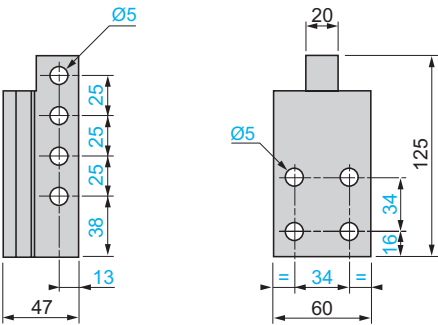
Right-angled connectors LA9 F2100 (set of 6) for rear connection
