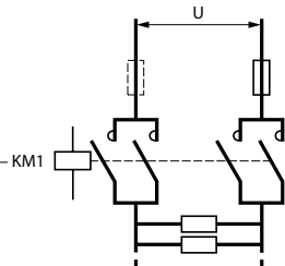
Circuit controlled by a 4-pole contactor with the poles parallel connected in pairs using appropriate connecting links. This solution enables the control of power values approximately equivalent to those controlled by the same contactor on 3-phase.
