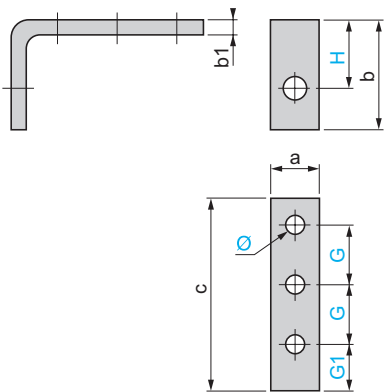
Right-angled connectors LA9 F●980 with large surface area (set of 3)
