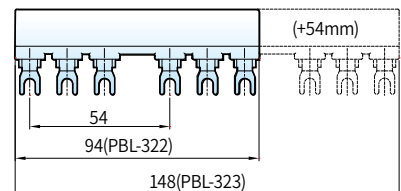
MMS-32H, HI+PBL-32 PBL-322(2 Terminal), PBL-323(3 Terminal)
