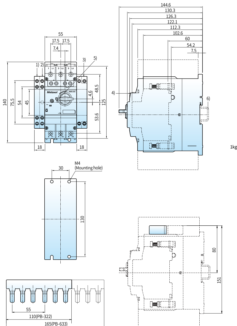
MMS-63S/H/HI+PB-63 PB-632 (2 Terminal), PB-633 (3 Terminal)
