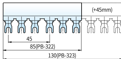
MMS-32H/HI+PB-32 PB-322 (2 Terminal), PB-323 (3 Terminal) PB-324 (4 Terminal), PB-325 (5 Terminal)
