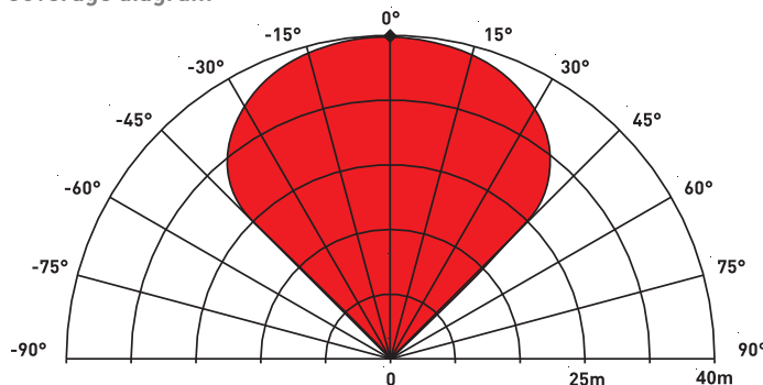
Coverage diagram
