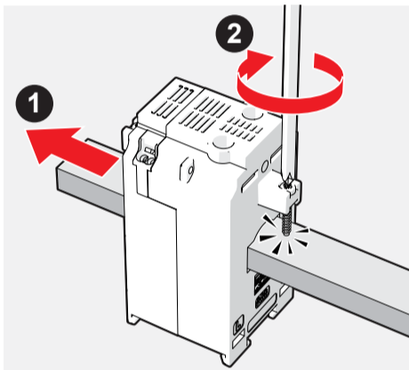
Installation on cable or primary busbar
