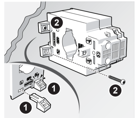
Wall-mounting installation
