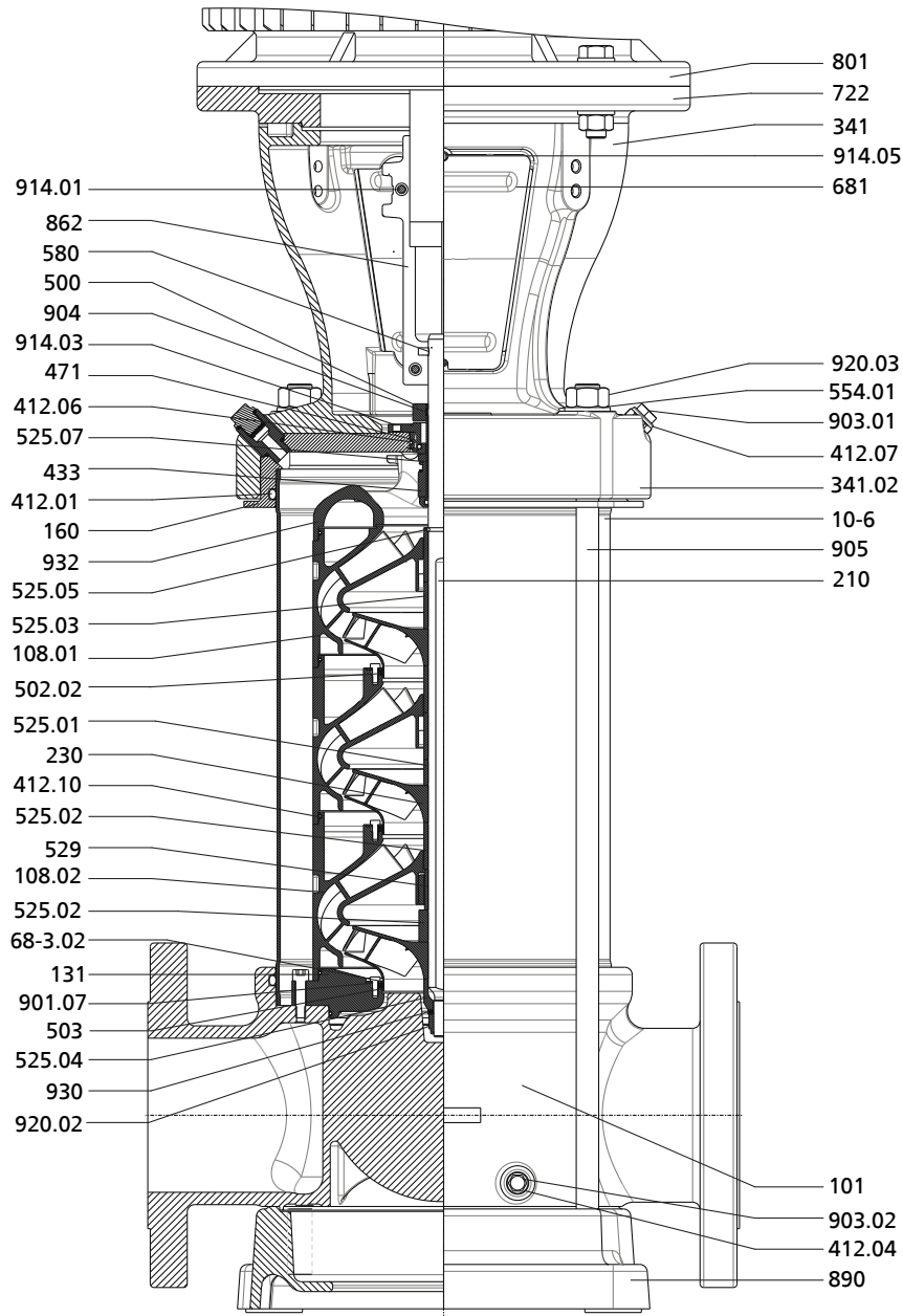
Fig. 80: General assembly drawing of Movitec 125B
