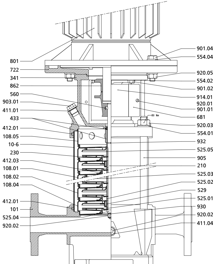
Fig. 81: General assembly drawing of Movitec LHS 6
