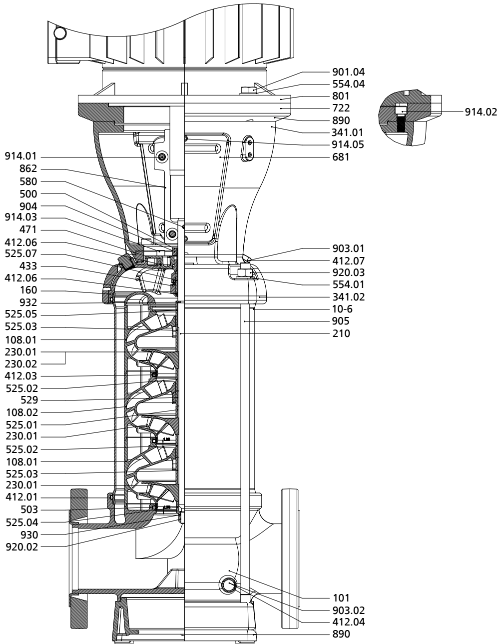
Fig. 79: General assembly drawing of Movitec 90B
