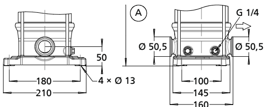
Fig. 6: Connections of Movitec VT, VST
