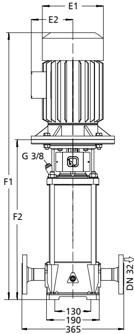
Dimensions of Movitec LHS6
