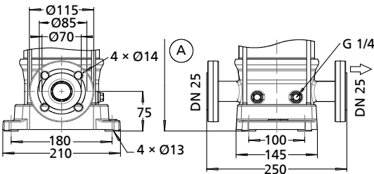
Fig. 13: Connections of Movitec VF, VSF
