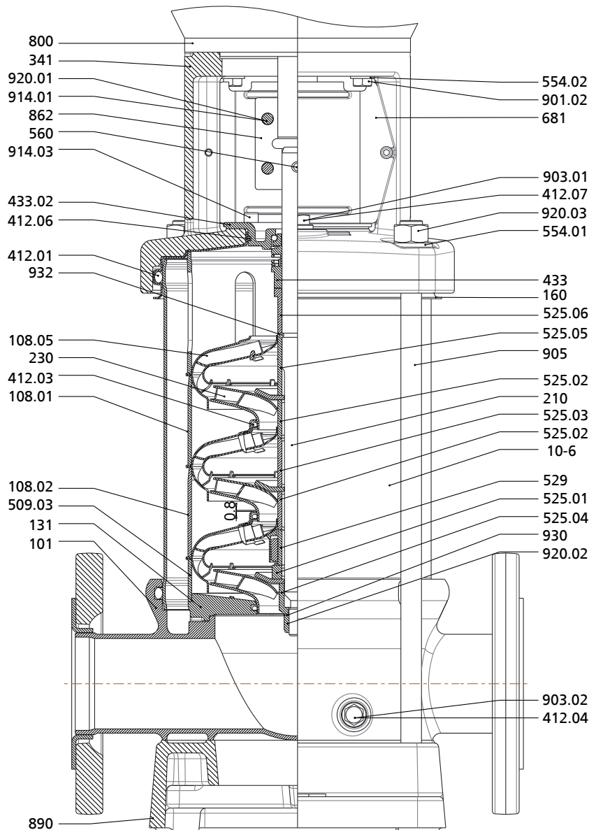
Fig. 78: General assembly drawing of Movitec 25B, 40B, 60B
