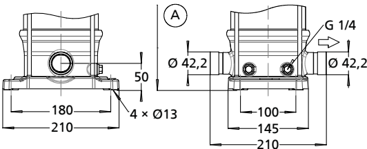
Fig. 11: Connections of Movitec VV, VSV
