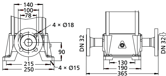
Fig. 70: Connections of Movitec LHS6
