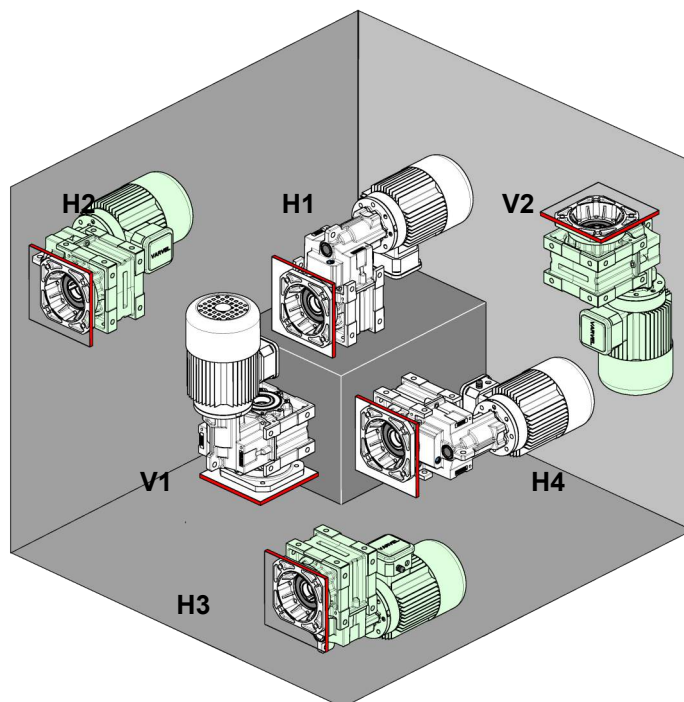
B5 Flange mounting
