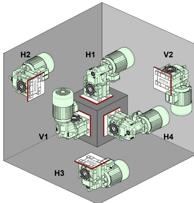
B3 Foot mounting
