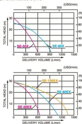
■ Performance Curve
