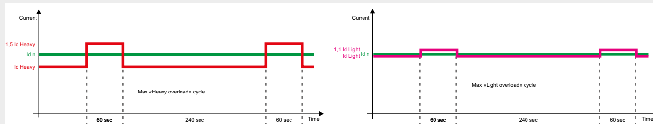
Overload curves
