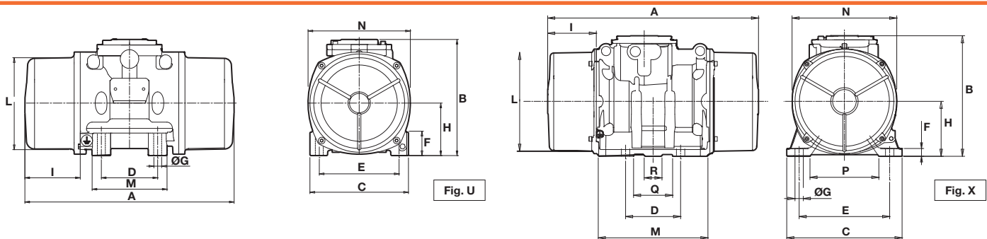
DIMENSIONAL SPECIFICATIONS (mm)
