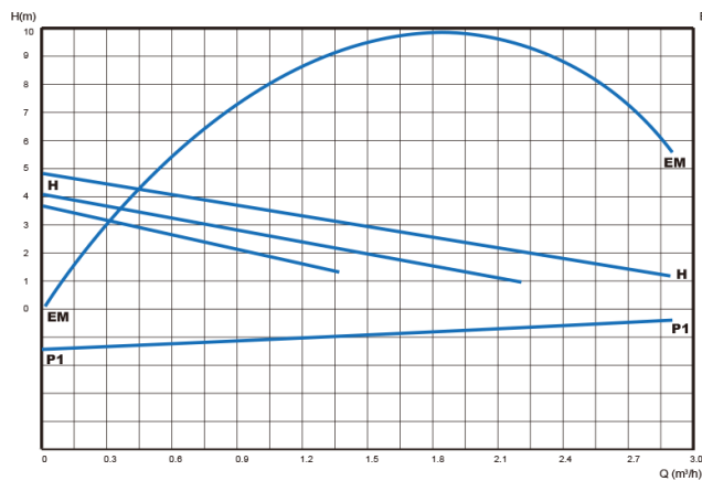
SXR25/4 PERFORMANCE CHART
