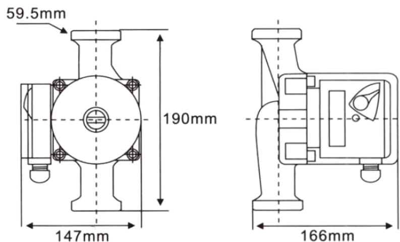
SXR32/8G INSTALLATION DEMENSION
