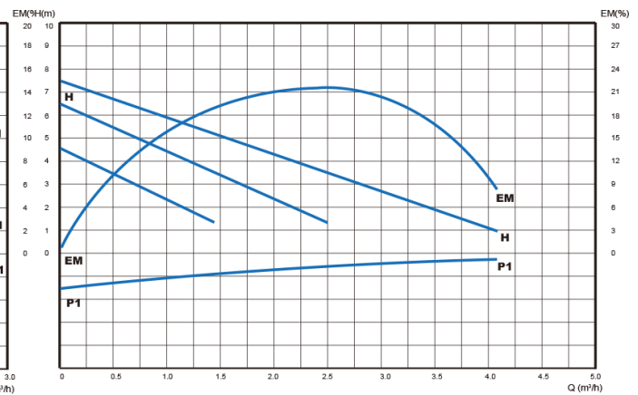
SXR25/7G PERFORMANCE CHART
