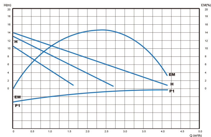
SXR25/15G PERFORMANCE CHART
