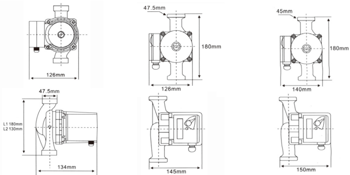
SXR25/4 INSTALLATION DIMENSIONS SXR25/7G INSTALLATION DIMENSIONS SXR25/15G INSTALLATION DIMENSIONS
