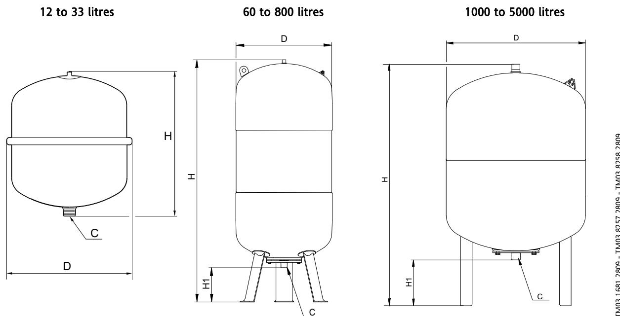
Fig. 6 Dimensional sketches
