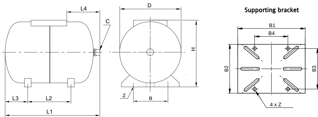
Fig. 11 Dimensional sketches
