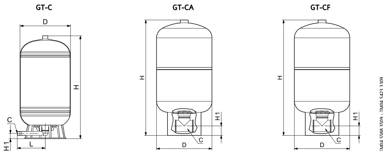
Fig. 13 Dimensional sketches
