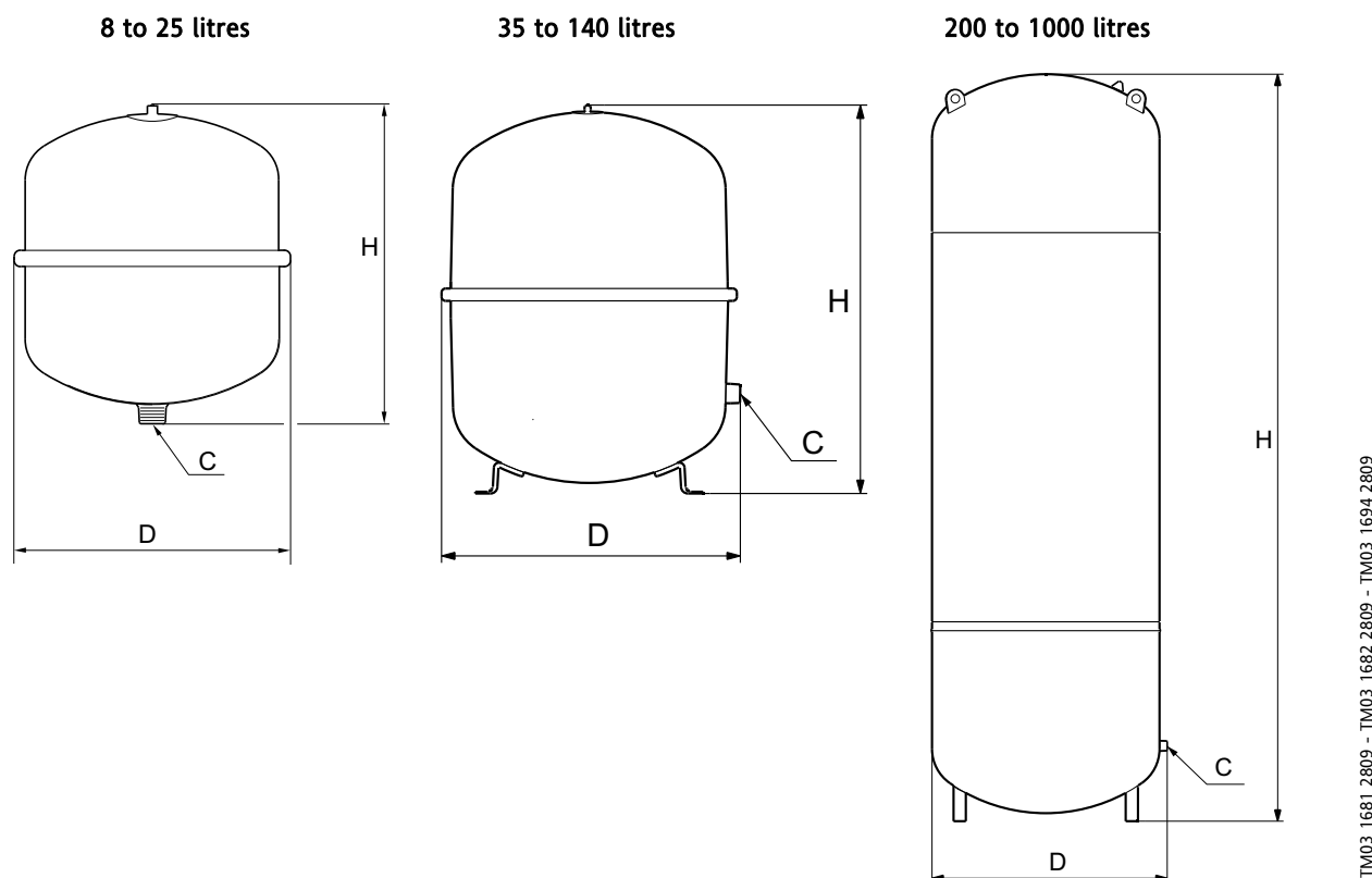
Fig. 14 Dimensional sketches
