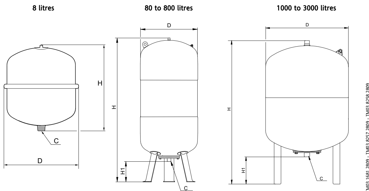
Fig. 8 Dimensional sketches
