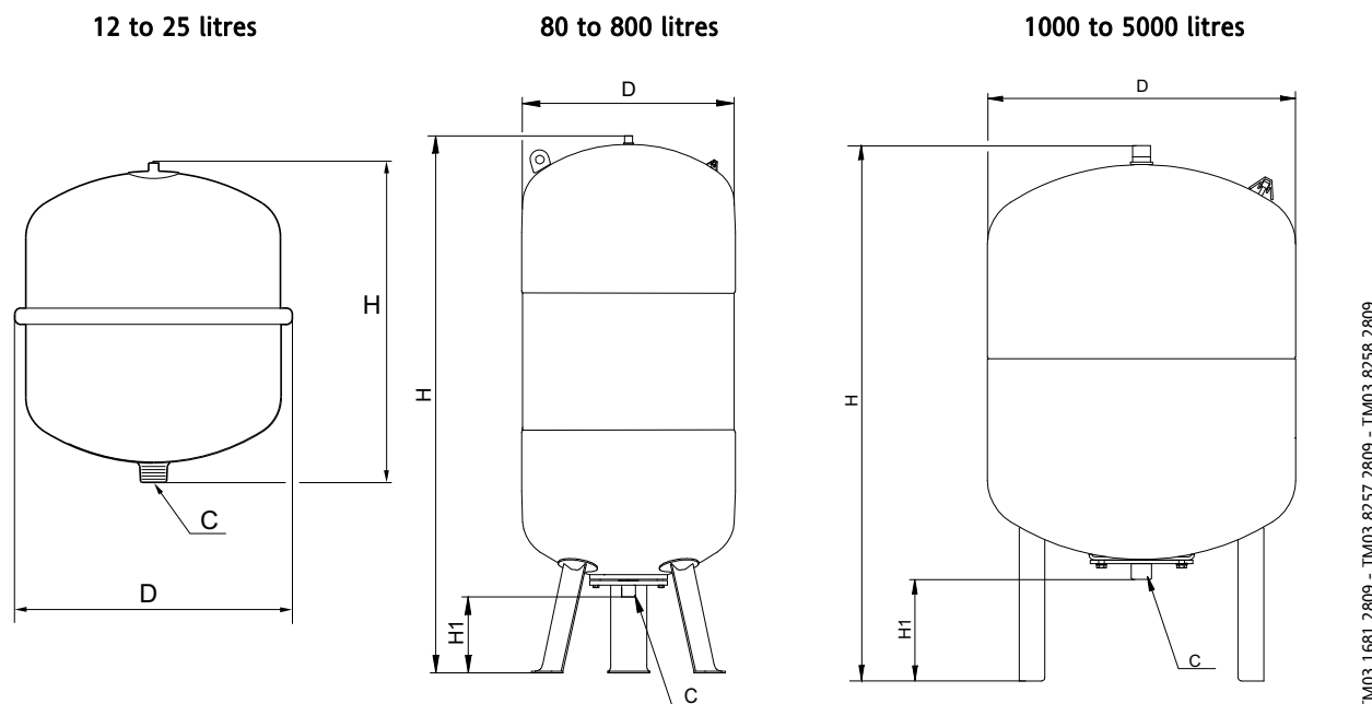
Fig. 7 Dimensional sketches
