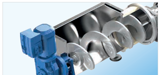
„coreless screw“ in WANGEN VarioTwin
